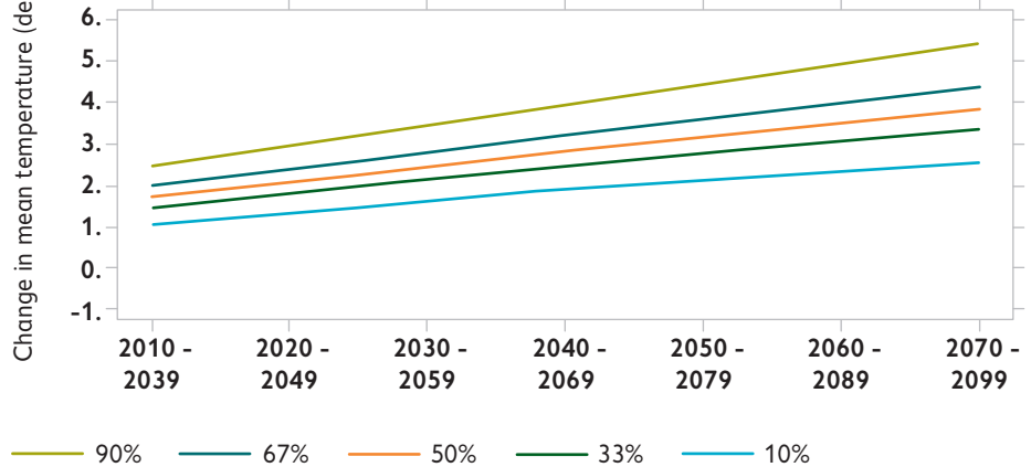
% probability of degrees Celsius Temperature change, based on a medium emissions scenario, SRES (UKCP09)
