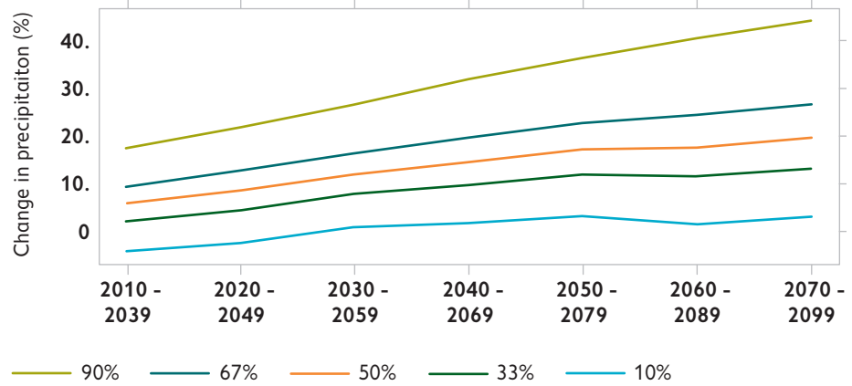
% probability of winter precipitation levels, based on a medium emissions scenario, SRES (UKCP09)
