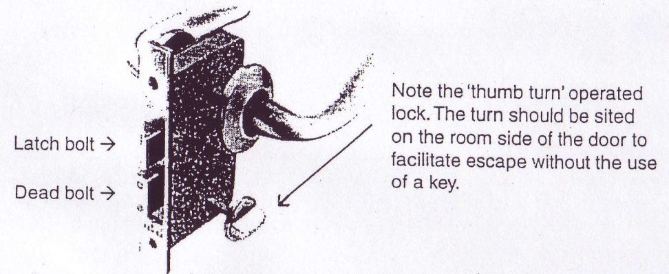
Figure 4.18 - Combined lock and latch unit
