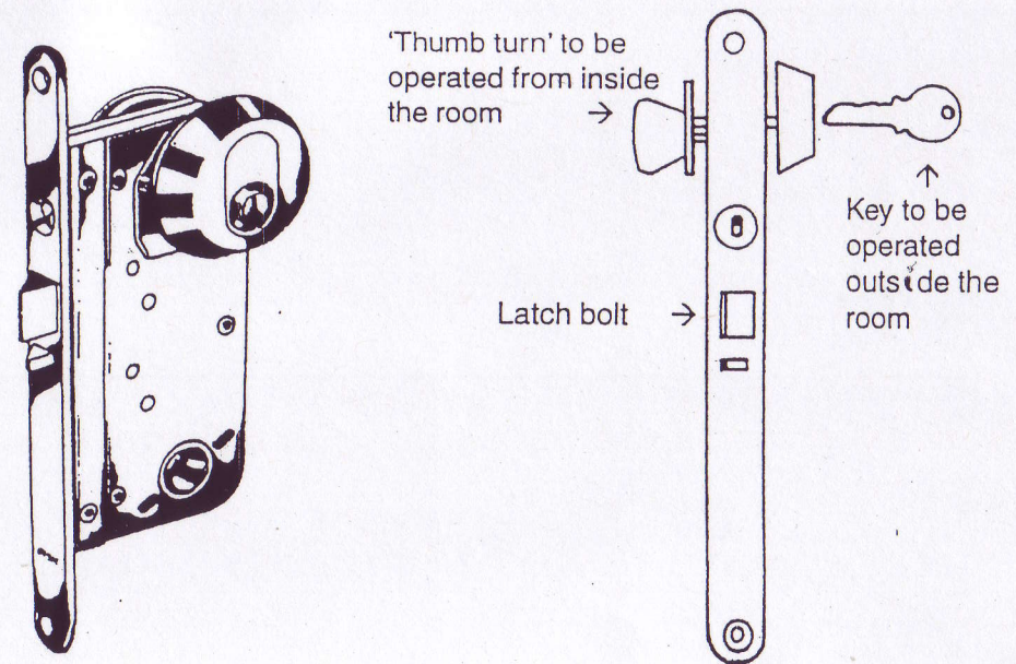
Figure 4.19 - Mortice Nightlatch
